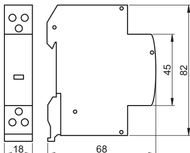
THK2-20
