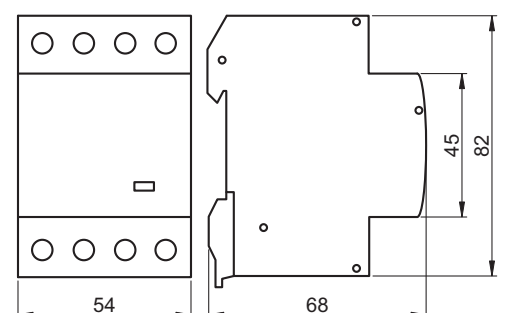
THK3-32, 3-40, 4-32, 4-40, 4-63
