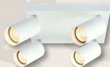
SPGU10MAN4W 220 × 220 × 125
